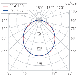
Light distribution curve for LINE SOLO (type O)
