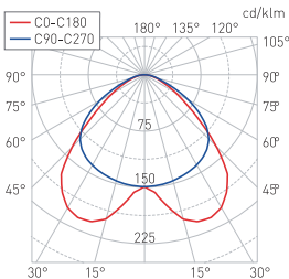
Light distribution curve for LINE SOLO (type MM)
