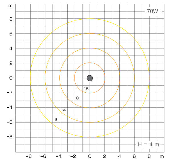
Luminous intensity diagrams, lx
