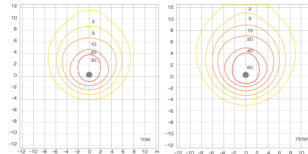
Luminous intensity diagrams, lx
