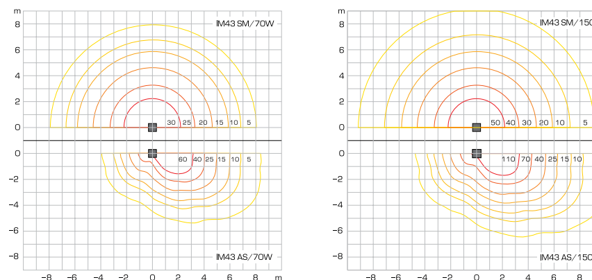
Luminous intensity diagrams, lx
