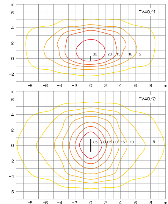
Luminous intensity diagrams, lx
